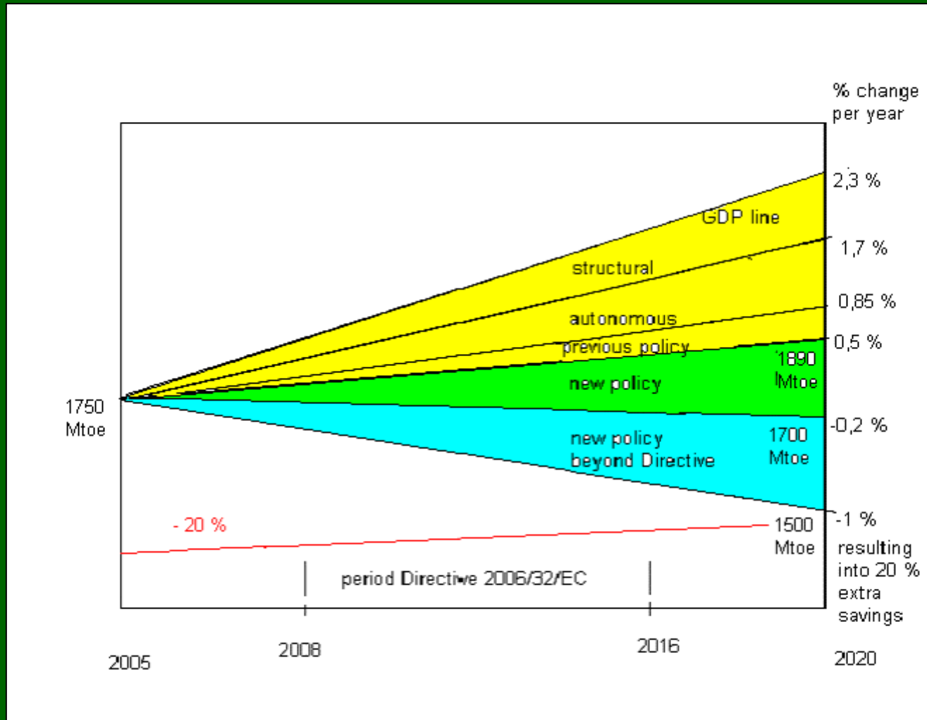
Figure 3: Annual improvements in energy intensity
